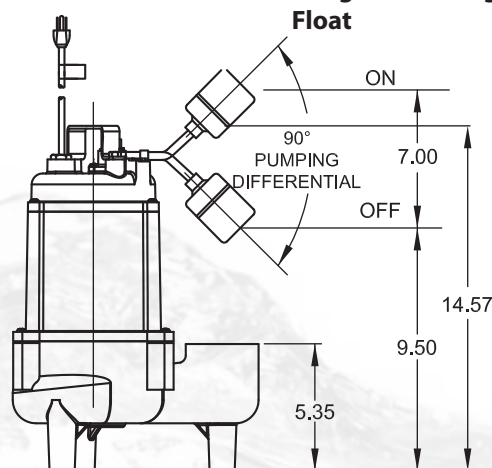
PFS531TWA1 with Integral wide angle Float
